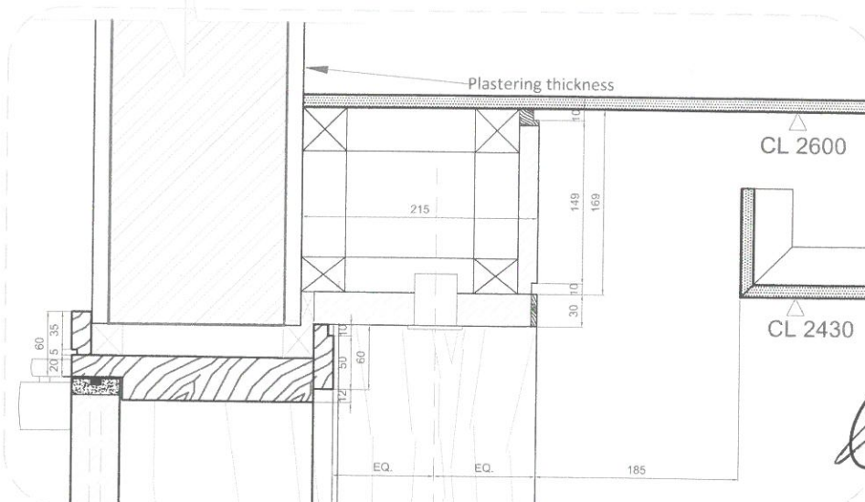
D1 Typical Bulkhead detail
