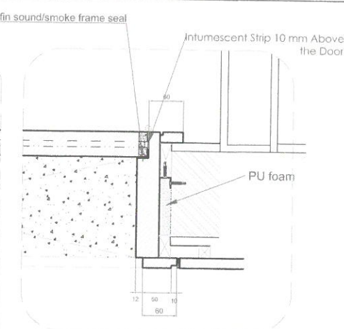
D4 Typical Frame detail
