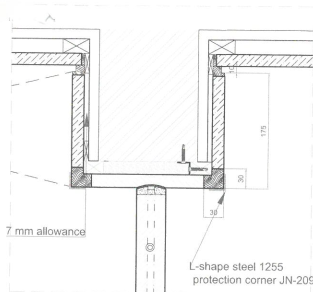
D5 Junction details
